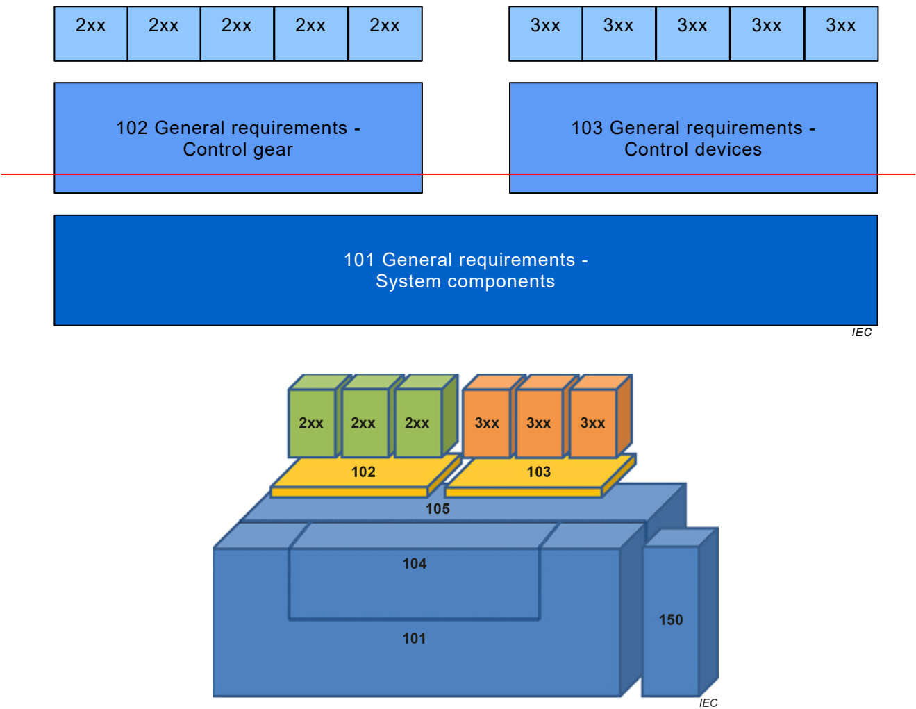
Figure 1 – IEC 62386 graphical overview
